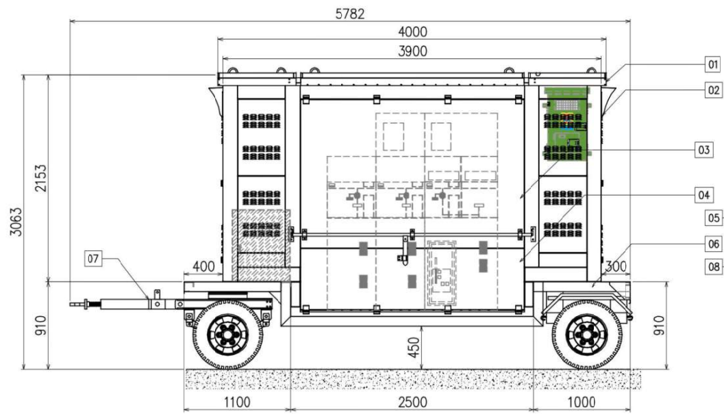
TAMPAK SAMPIING
